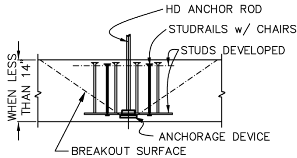
SECTION ELEVATED SLAB NTS
