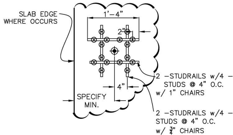
PLAN VIEW ELEVATED SLAB NTS
